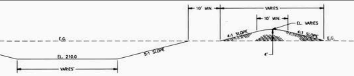
TYPICAL SECTION OF PONDS 1 & 2 NOT TO SCALE
