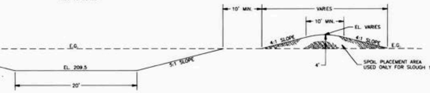
TYPICAL SECTION OF SLOUGH 1 NOT TO SCALE
