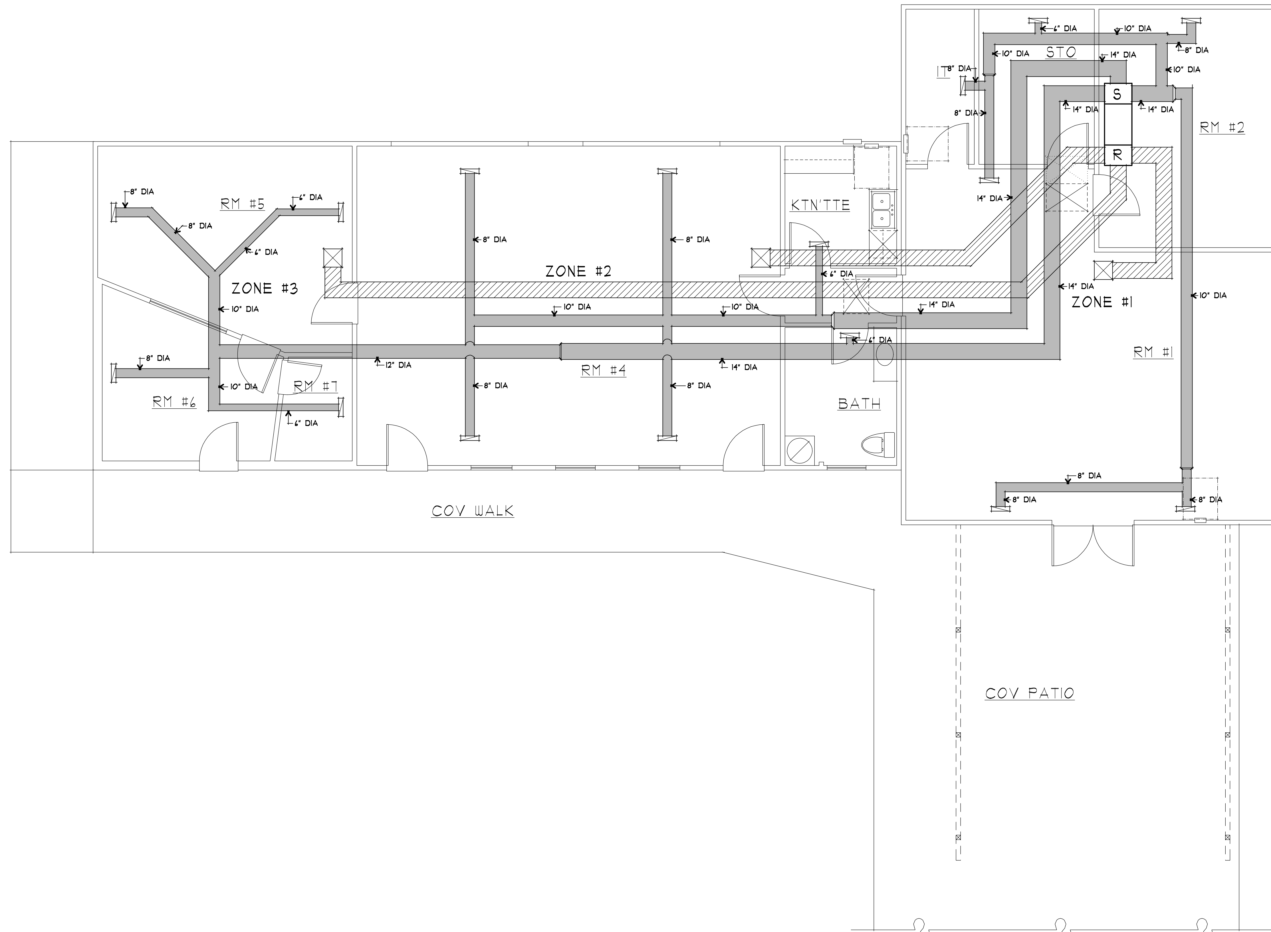
1 HEATING PLAN @ STUDIO 6 1/4" = 1'-0"
