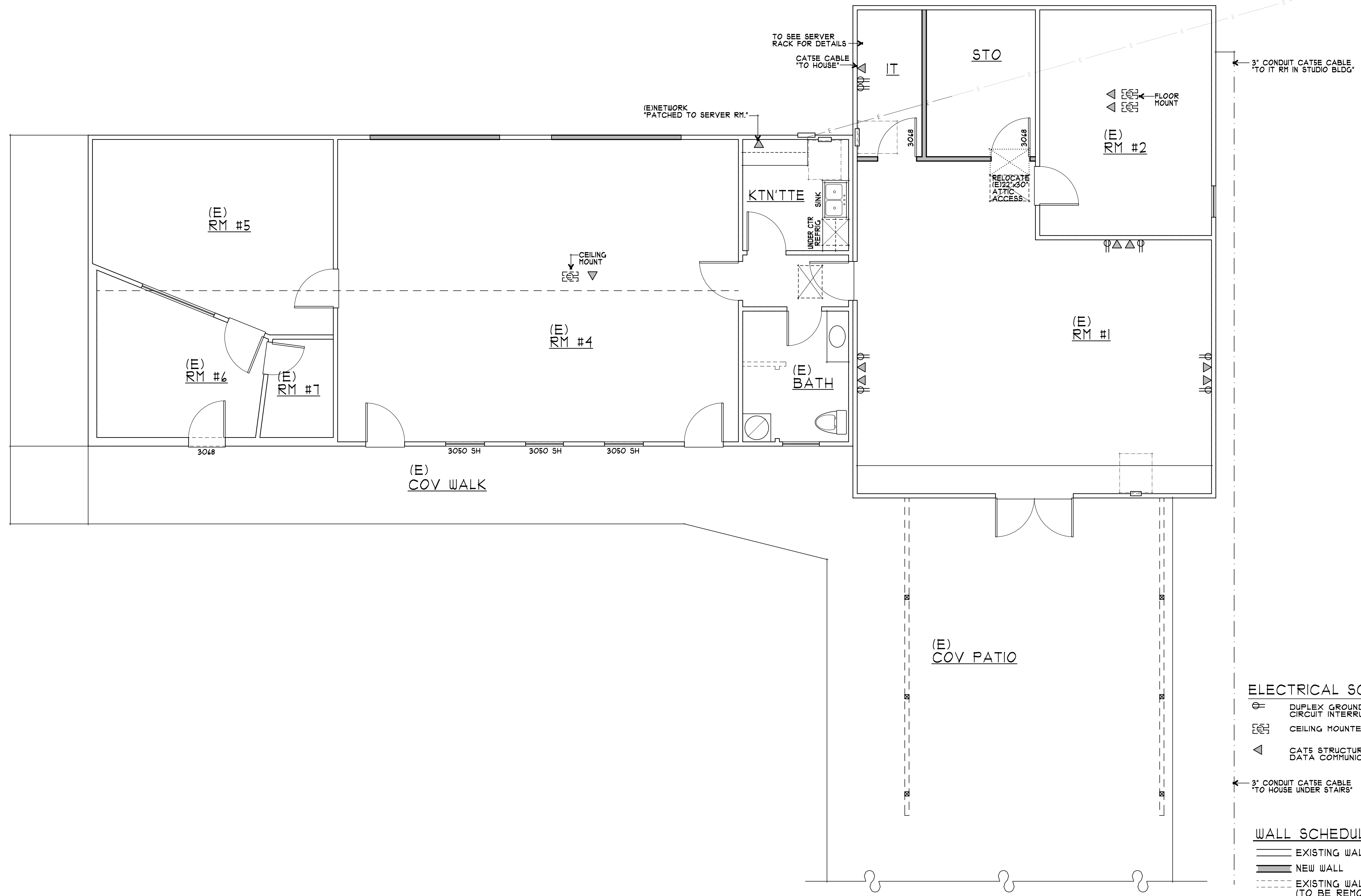
1 4 NEW FLOOR PLAN @ STUDIO 1/4" = 1'-0"
