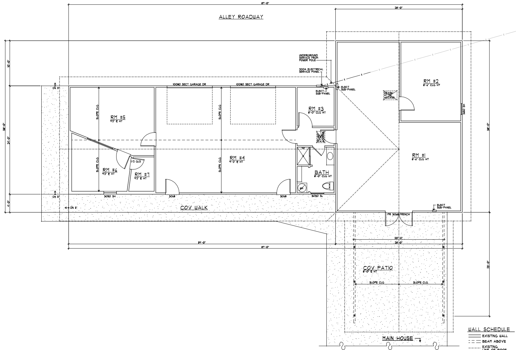
1 2 EXISTING FLOOR PLAN @ STUDIO 1/4" = 1'-0"
